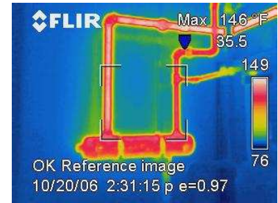
Hot Water Systems
